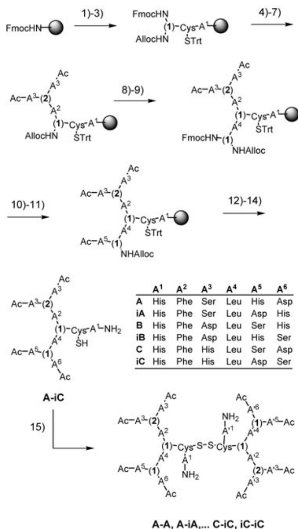
Scheme 3. Solid phase synthesis of peptide dendrimers. Conditions: Deprotecting steps: i = DMF, piperidine (4:1); ii = PhSiH 3 (25 equivs.), CH 2 Cl 2 , 3 min, then Pd(PPh 3 ) 4 (0.1 equiv.). Coupling steps: iii = BOP/DIEA. Capping steps: iv = Ac 2 O/CH 2 Cl 2 (1:1). 1) i, then iii with FmocA 1 OH; 2) i, then iii with FmocCys(Trt)OH; 3) i, then iii with 1 ; 4) i, then iii with FmocA 2 OH; 5) i, then iii with 2 ; 6) i, then iii with FmocA 3 OH; 7) i, then iv; 8) ii, then iii with FmocA 4 OH; 9) i, then iii with 1 ; 10) i, then iii with FmocA 5 OH; 11) i, then iv; 12) ii, then iii with FmocA 6 OH; 13) i, then iv; 14) TFA cleavage and HPLC purification; 15) disulfide coupling with 2,2'-dithiopyridine.
