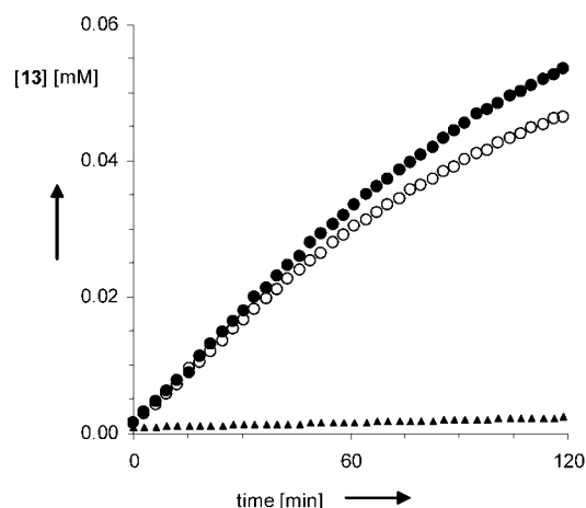
Figure 1. Time-course graph for the hydrolysis of 10 to form 13 in the absence ( \blacktriangle ) or presence of dendrimers iA–iC ( \bullet ), or iA–C ( \circ ). Conditions: 200 \mu\text{M} substrate 10 , 5 \mu\text{M} dendrimer, 26 ^{\circ}\text{C} , in 20 mM aqueous bis-Tris buffer pH 6.0. The reaction was followed using a SpectraMAX fluorescence plate reader ( \lambda_{\text{exc}} = 460 \text{ nm} , \lambda_{\text{em}} = 530 \text{ nm} ). Fluorescence was converted to product concentration using a calibration curve, which was linear in the concentration range used.
