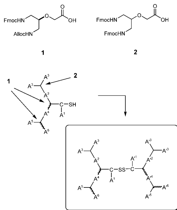
Scheme 1. Structure of disulfide-bridged peptide dendrimers with differential functionalization of layers. (A 1 –A 6 , A 1' –A 6' =variable amino acids, C=cysteine).
