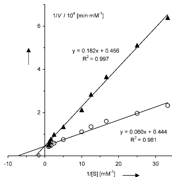
Figure 2. Double reciprocal plot for hydrolysis of ester 10 catalyzed by peptide dendrimers iC–iC (HHSD–HHSD) ( \circ ) and iA–iC (DDHS–HHDS) ( \blacktriangle ).
