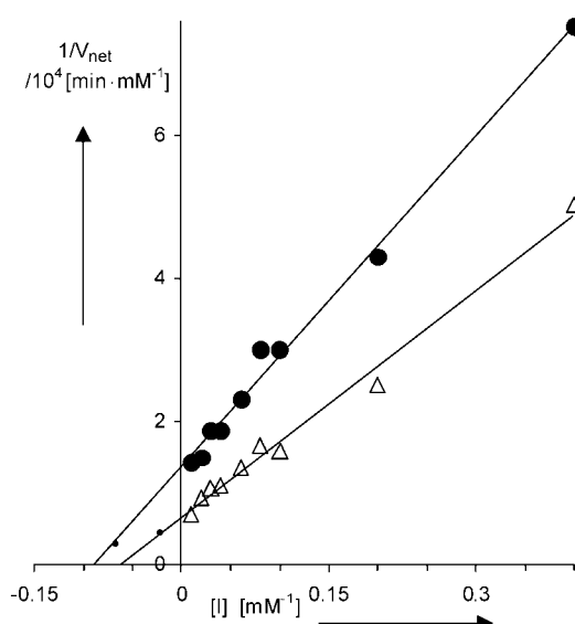
Figure 3. Dixon plot for competitive inhibition of dendrimer-catalyzed hydrolysis of acetate ester 9 by 1,3,6,8-pyrene-tetrasulfonate 14 . Measured in 20 mM bis-Tris pH 6.0, 0.2 mM 9 , and dendrimer C (●), and dendrimer CC (Δ). The competitive inhibition constant is the x-coordinate of the intercept between the fitted lines and the horizontal lines drawn at y = 1/V_{\text{max}} .
