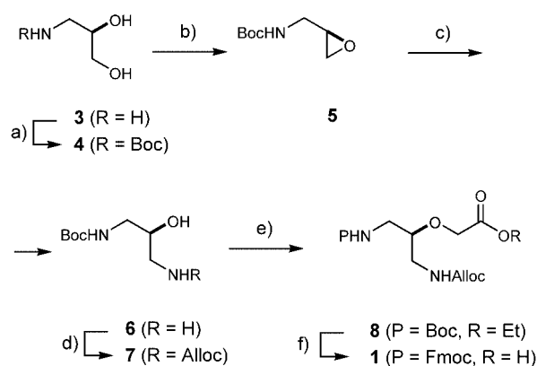
Scheme 2. Synthesis of chiral branching unit 1 . Conditions: a) Boc 2 O, Et 3 N, CH 2 Cl 2 /MeOH, 2 h, 25 °C, 94%; b) MsCl, Pyr, 0 °C, then NaOH, DMSO, 0 °C, 74%; c) NH 4 OH, EtOH, 1.5 h, quant.; d) allyl chloroformate, EtOAc, NaHCO 3 , 4 h, 87%; e) BrCH 2 CO 2 Et, NaH, dry THF, 5 h, 63%; f) i) LiOH, THF/H 2 O, 25 °C, overnight, ii) aqueous 3 N HCl, 60 °C, 3 h, iii) Fmoc-Cl, NaHCO 3 , H 2 O/dioxane, 25 °C, overnight, 63%. Boc = tert -butoxycarbonyl, THF = tetrahydrofuran, Fmoc-Cl = 9-fluorenylmethoxycarbonyl chloride, MsCl = methanesulfonyl chloride.
