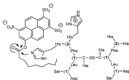
Figure 4. Hydrolysis of 8-nonyloxy-1,3,6-trisulfonate 10 by catalytic peptide dendrimer CC involves electrostatic and hydrophobic substrate binding and nucleophilic catalysis by histidine side-chains.
