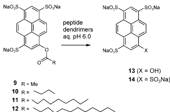
Scheme 4. The hydrolysis of pyrene 1,3,5-trisulfonate esters is catalyzed by hydrophobic core peptide dendrimers with surface catalytic residues.
